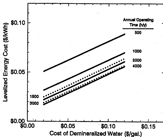
Figure 3. Parametric Analysis of Levelized Energy Cost for Set Operating Hours as Functions of Water Treatment Costs
